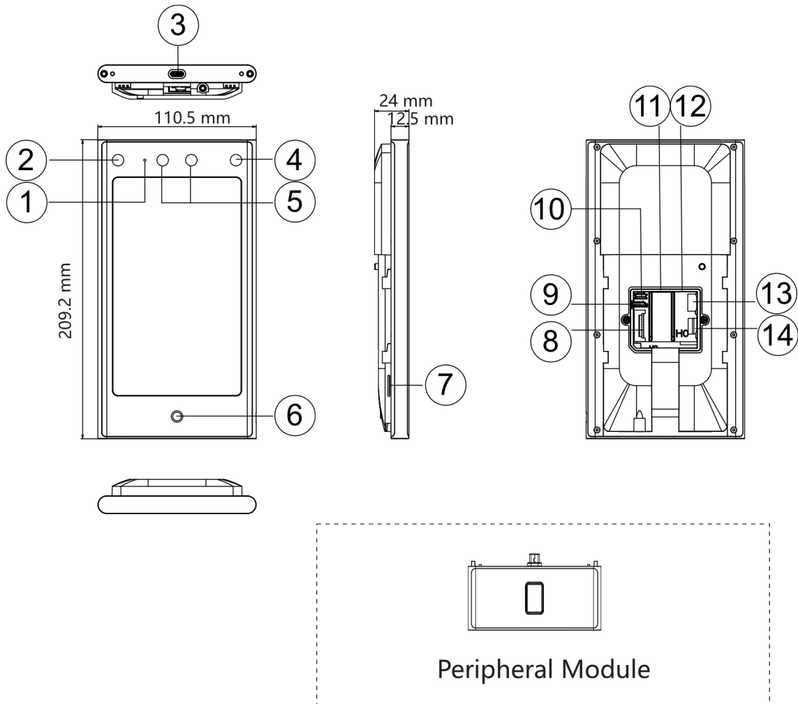
Figure 2-1 Face Recognition Terminal Diagram
